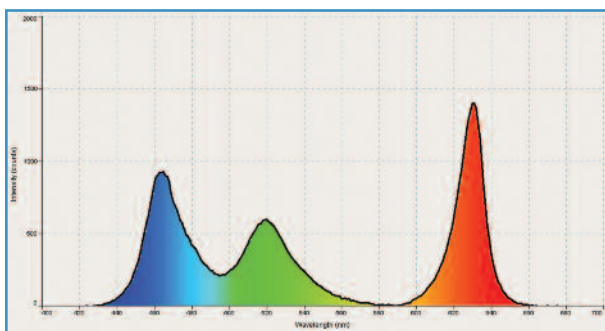
Figure 4: Spectrum—RGB
