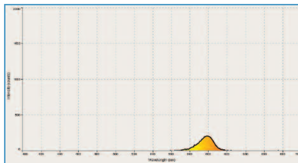
Figure 5: Spectrum—amber
