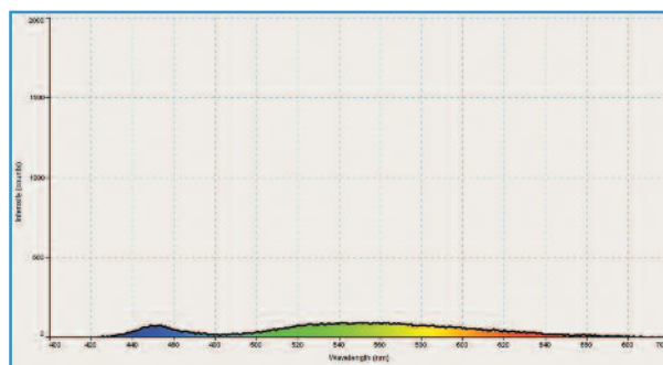
Figure 6: Spectrum—white
